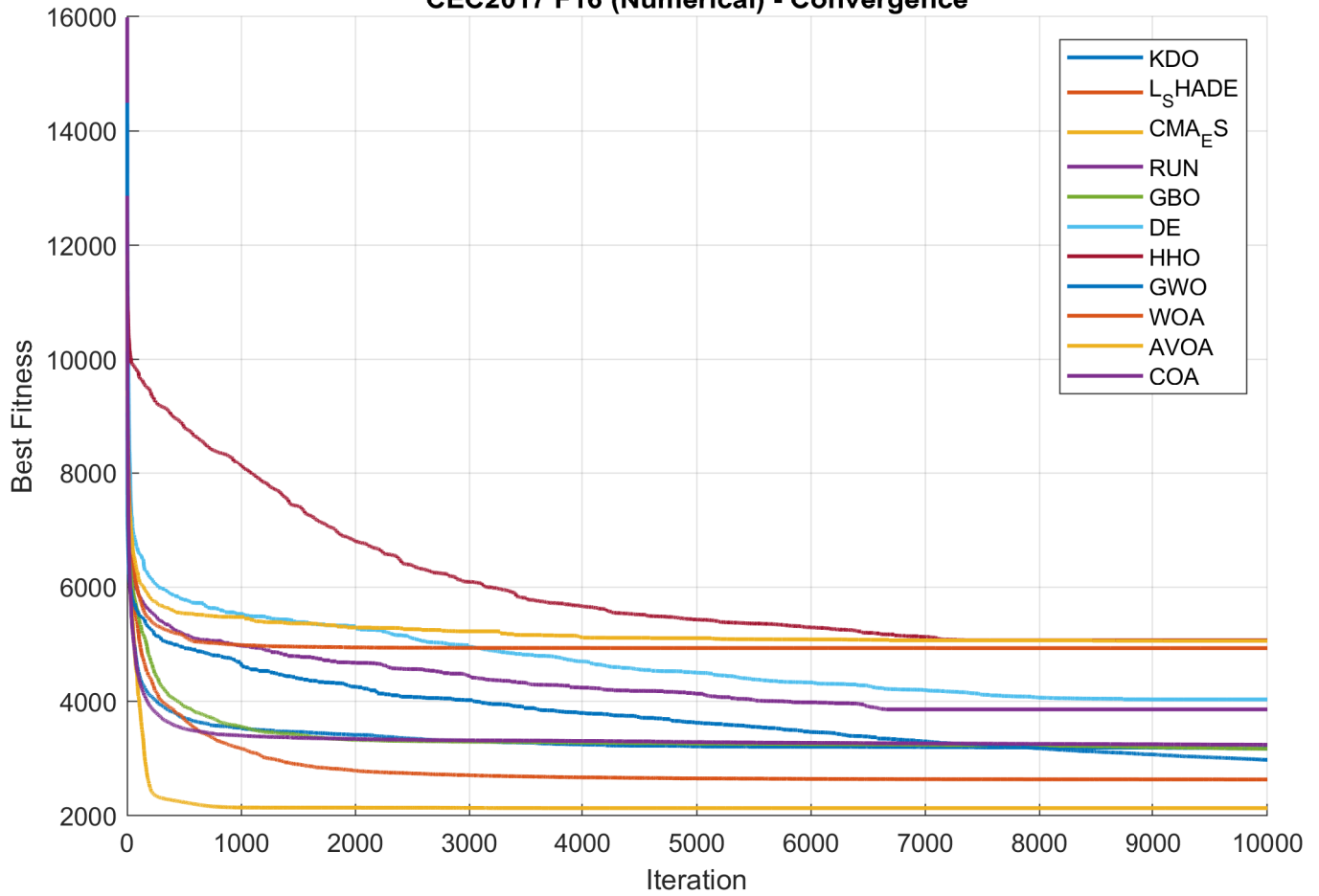
CEC2017 F16 (Numerical) - Convergence
